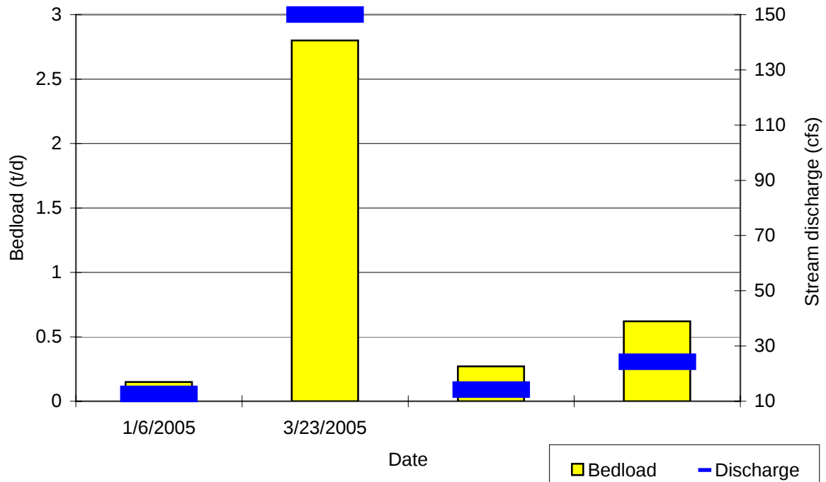
Figure 20.--Measured stream discharge and bedload sediment for site CC1, Camp Creek at Alabama Highway 253, Marion County, Alabama.
