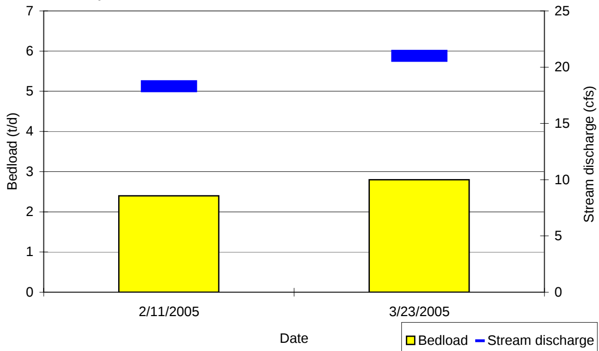
Figure 21.--Measured stream discharge and bedload sediment for site PM1, Pearces Mill Creek at Alabama Highway 253, Marion County, Alabama.
